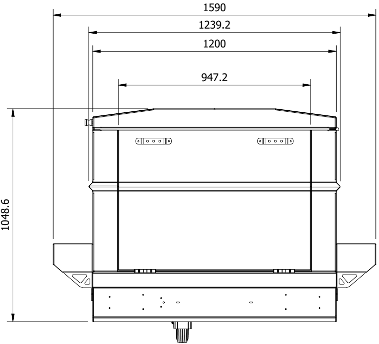
VIEW A SCALE ( 1 : 19 ) Back View
