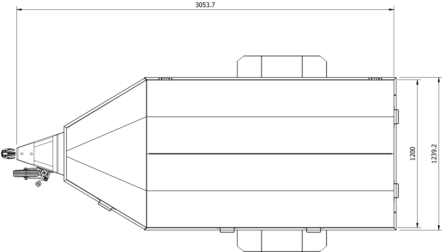
VIEW B SCALE ( 1 : 19 )
