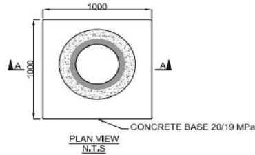
STANDARD CONCRETE ROUND BIN WITH CANOPY STANDARD SIZE N.T.S
