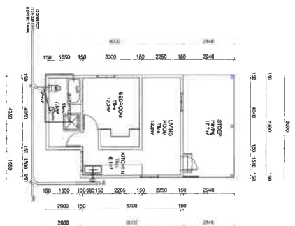
WORKERS HOUSE GROUND FLOOR PLAN: Scale 1:100
